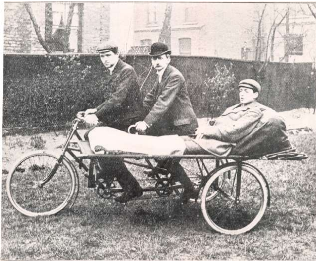
Tandem pattern of Patent Cycle Ambulance.
